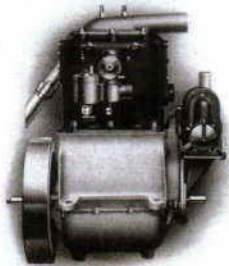
Showing side view of Swift Cyclecar water-cooled engine, from which it will be noticed that the carburetor and magneto are fitted in such positions as to be easily accessible.
