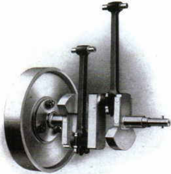
Cyclocar crankshaft with connecting rods and flywheel, the large diameter of the latter being at once noticeable.
