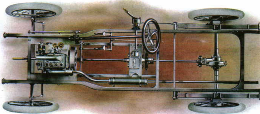
PLAN VIEW OF CYCLECAR CHASSIS
