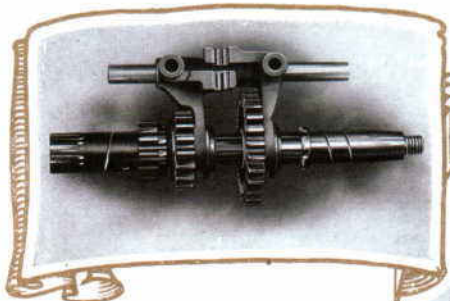
General and sectional views of three-speed gear box. All gears and gear shafts are cut from the solid, and are of the finest steel, case hardened. The box itself is aluminium, and cast in one piece, thus removing all possibility of leakage.
