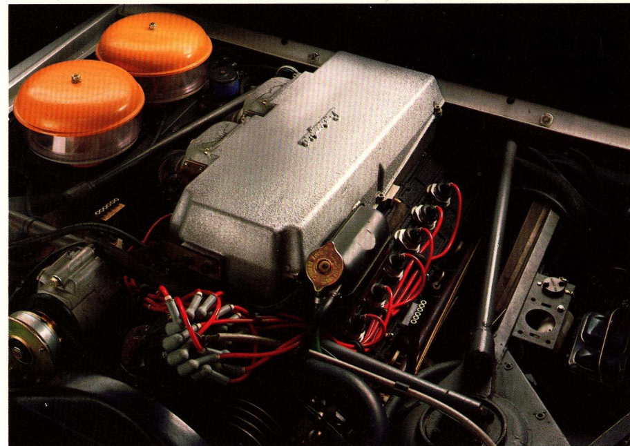
The LM002 standard 48-valve V-12 engine produces 455 hp @ 7,000 rpm.
