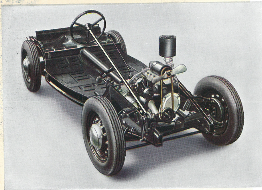
The Chassis.—Strength scientifically achieved without undue weight.
