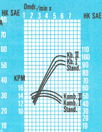
Effektdiagram for MORRIS Monaco mk. II
