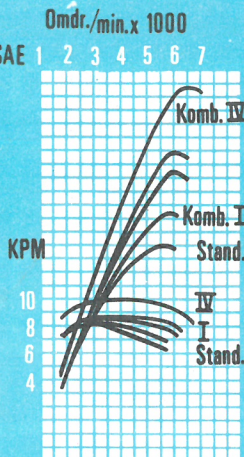
Effektdiagram for MORRIS Mascot Super (998 cc)
