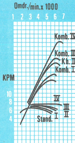
Effektdiagram for MORRIS Mascot 850 cc
