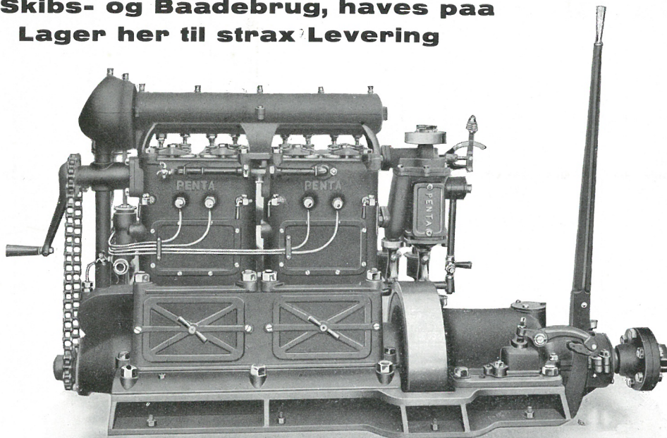
24 HK. 4-cylindret Penta Marin Motor
